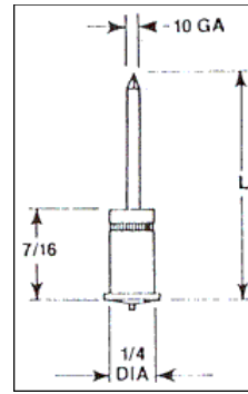
PIN BI-METALLIC
